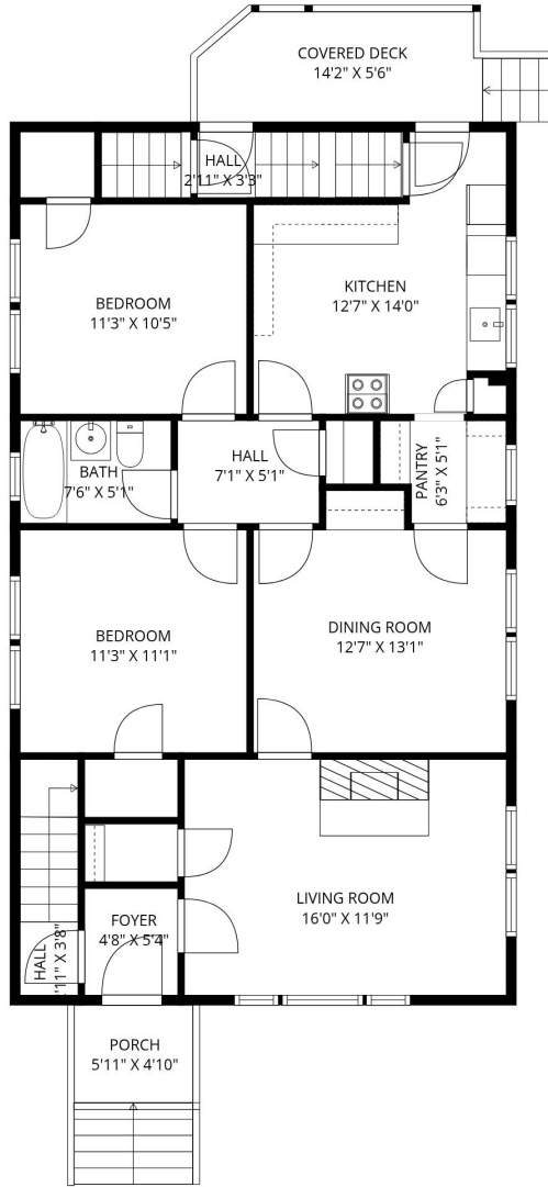
1ST FLOOR
